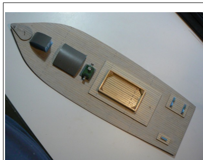
Implantations fixes
